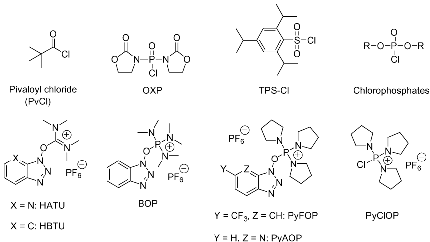
Figure 1. Condensing agents used for the coupling of 1 and 2 (for R see text or Table 1).
